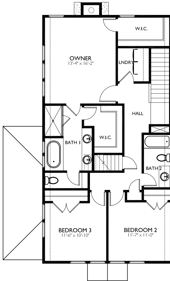
3RD FLOOR 9'-0" CLGs
