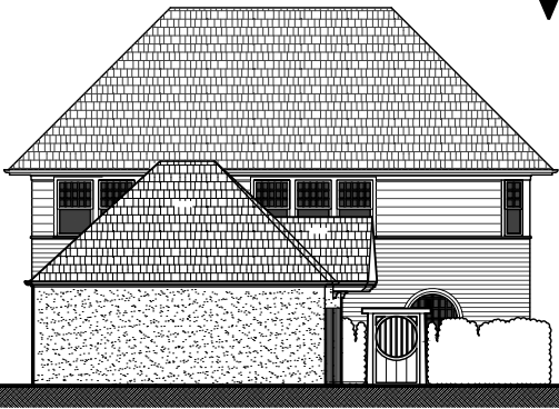
DRIVEWAY ELEVATION
