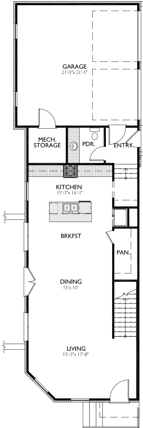
1ST FLOOR 10'-0" CLGs
