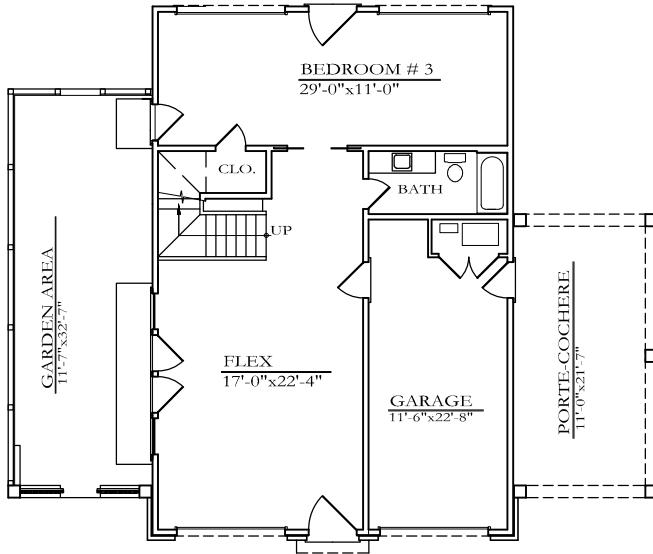
LOWER LEVEL FLOOR PLAN 9'-0" CEILING
