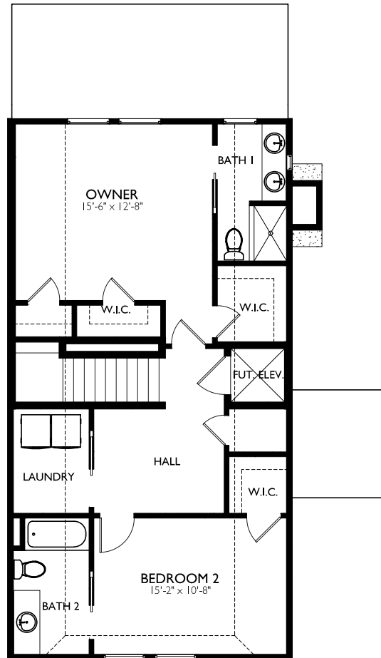
3RD FLOOR 7'-0" VAULTED TO 11'-0" CLGs
