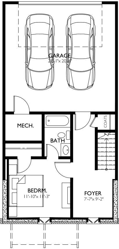
BASEMENT 8'-0" CLGs
