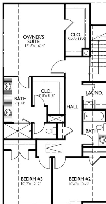
3RD FLOOR 9'-0" CLGs
