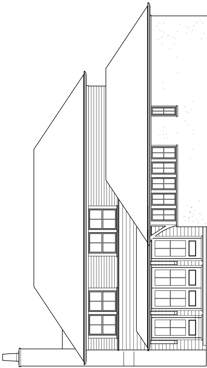
FRONT ELEVATION
