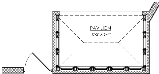
GARDEN PAVILION PLAN
