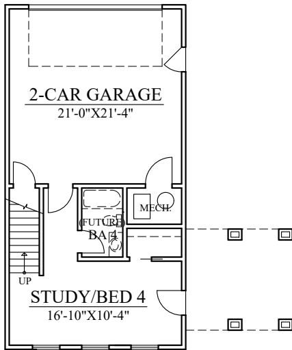
TERRACE FLOOR PLAN 8'-0"+ CEILING
