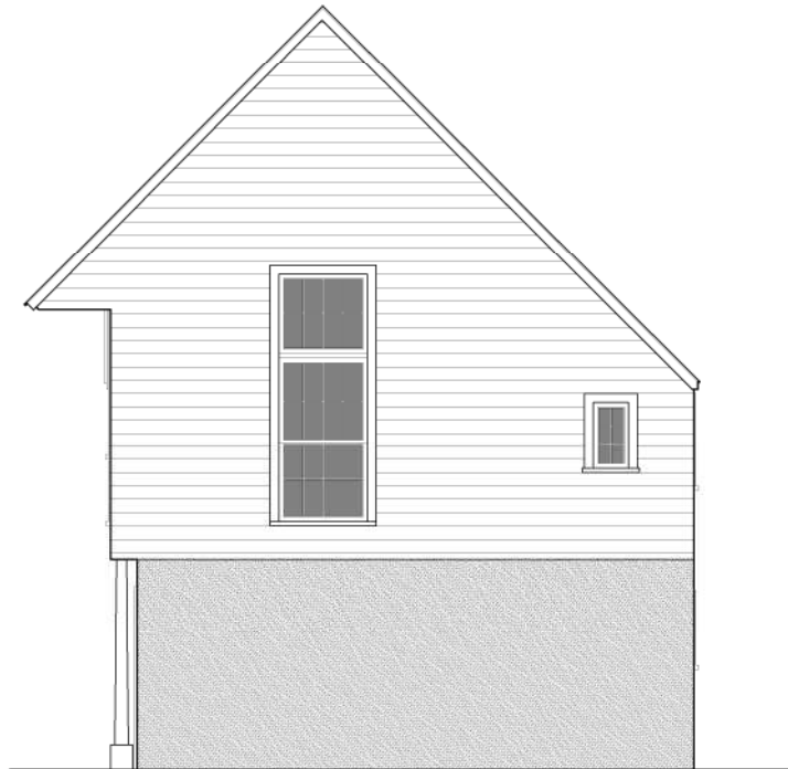
GARAGE RIGHT ELEVATION
