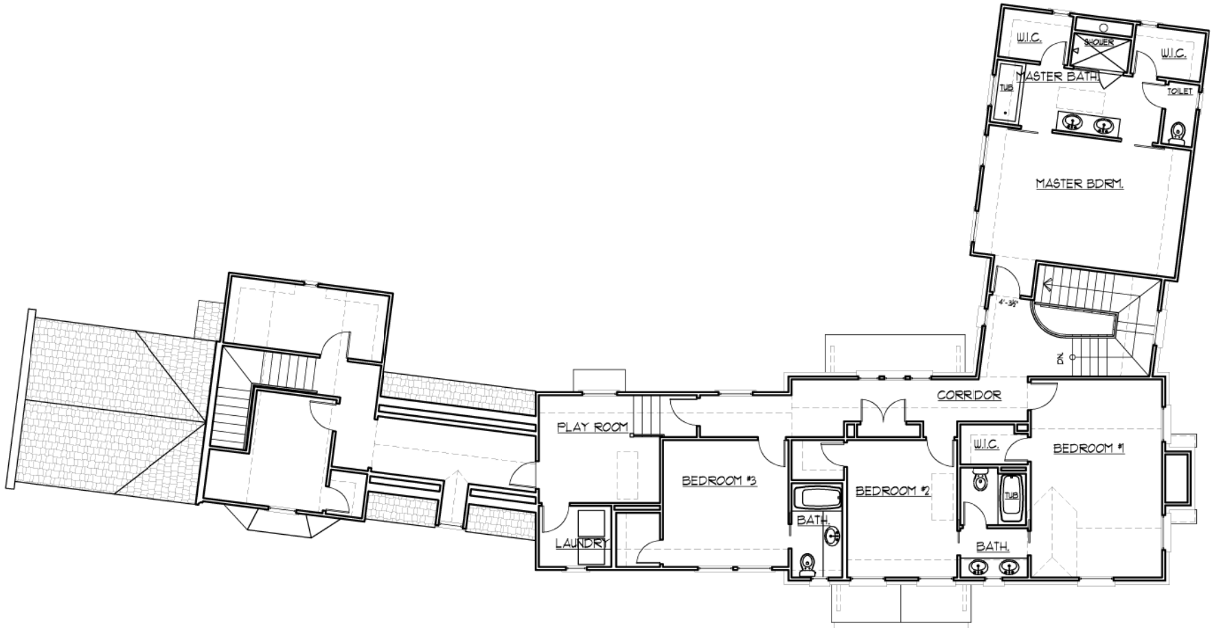
MAIN HOUSE UPPER FLOOR PLAN 9'-0"/13'-0"/10'-0" CEILINGS
