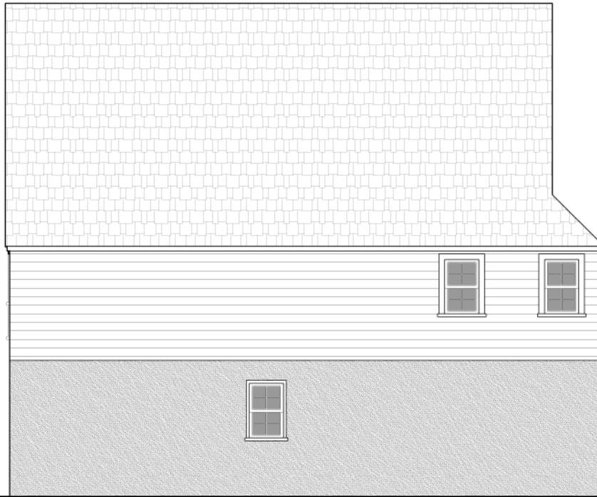
GARAGE REAR ELEVATION
