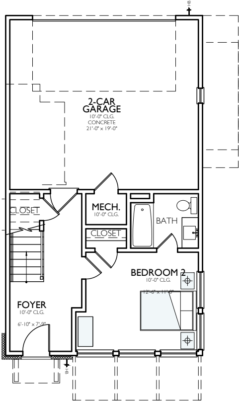
1ST FLOOR 10'-0" CLGS
