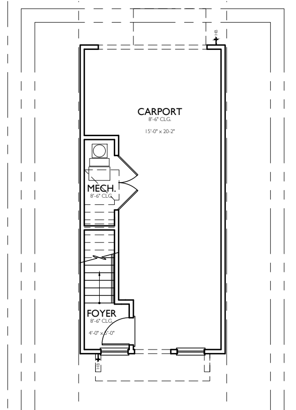
1 ST FLOOR 8'-6" CLGS
