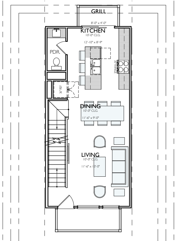
2ND FLOOR 10'-0" CLGS
