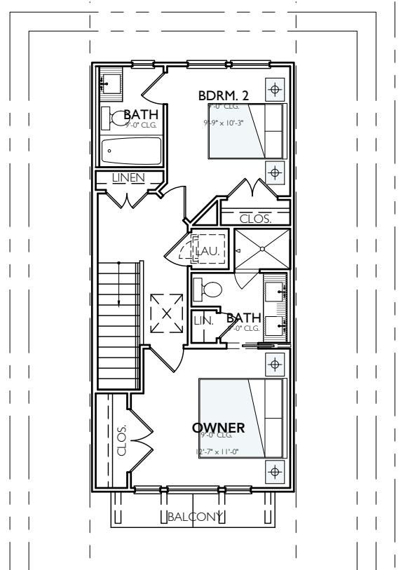
3RD FLOOR 9'-0" CLGS
