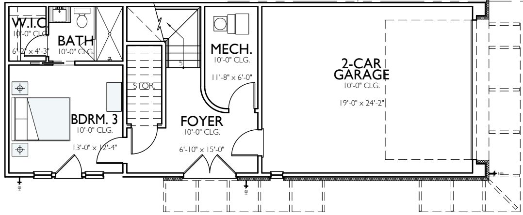
1ST FLOOR 10'-0" CLGS
