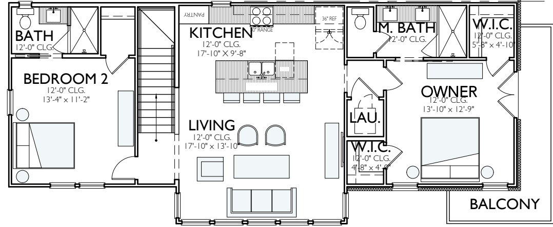
2ND FLOOR 12'-0" CLGS
