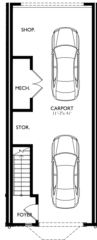
1ST FLOOR 8'-0" CLGs
