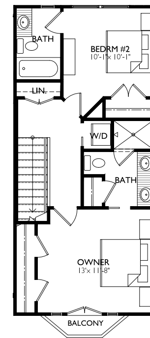
3RD FLOOR 9'-0" CLGs
