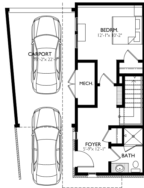
1ST FLOOR 8'-0" CLGs
