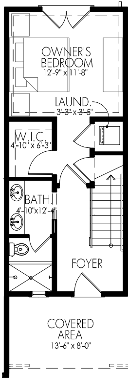
1ST FLOOR 8'-0" CLGs
