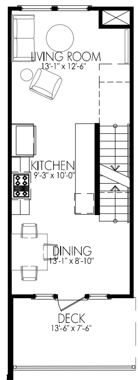
2ND FLOOR 10'-0" CLGs
