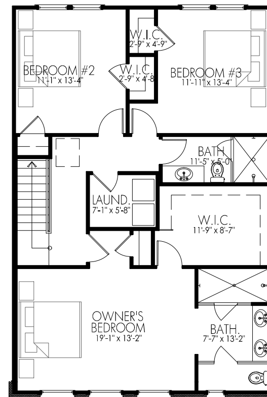
3RD FLOOR 9'-0" CLGs
