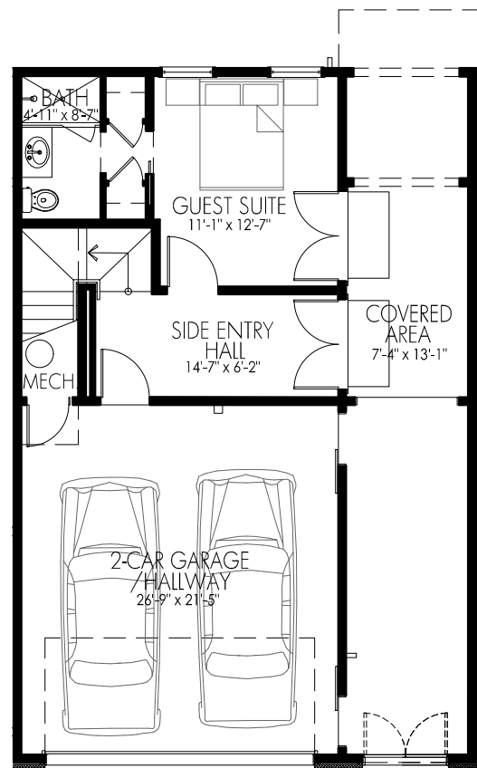
1ST FLOOR 8'-0" CLGs
