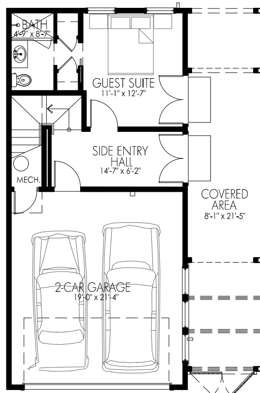
1ST FLOOR 8'-0" CLGs
