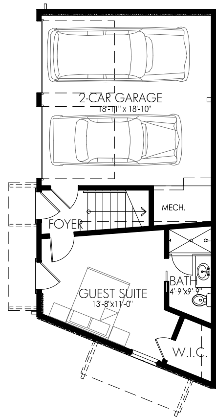
1ST FLOOR 8'-0" CLGs
