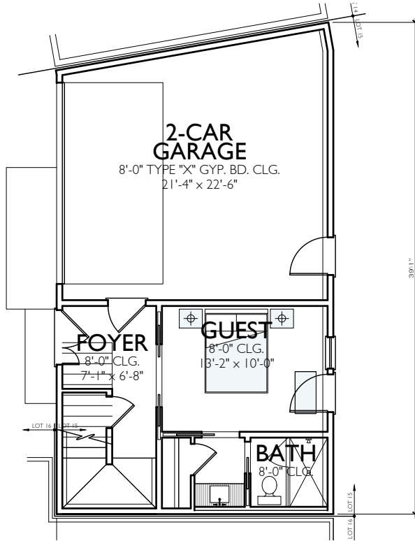
1ST FLOOR 8'-0" CLGs
