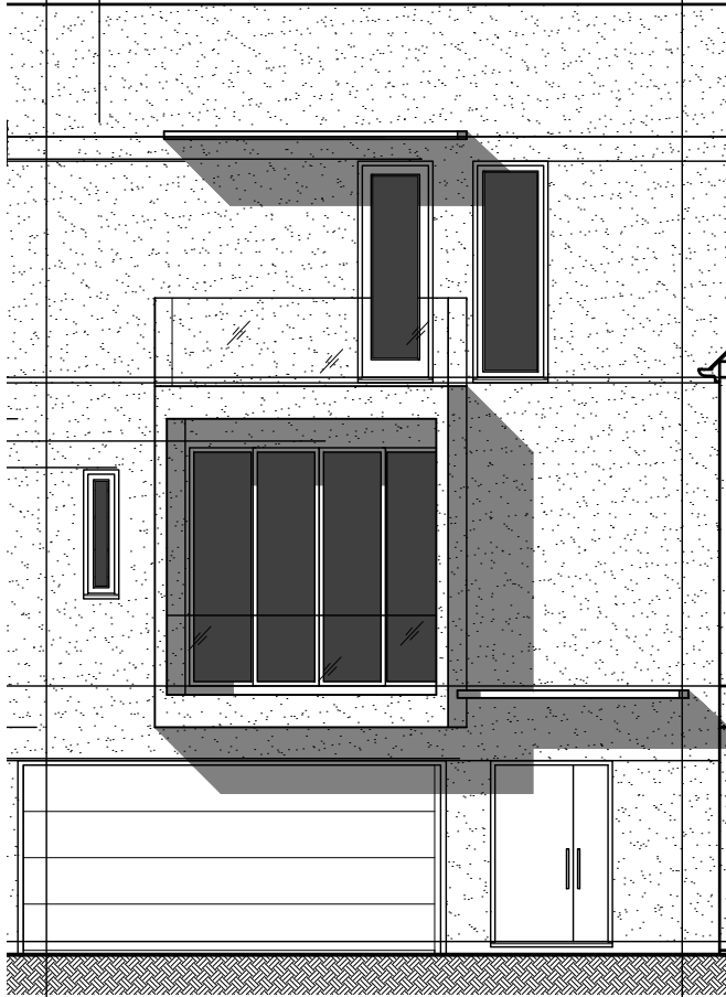
COURTYARD ELEVATION
