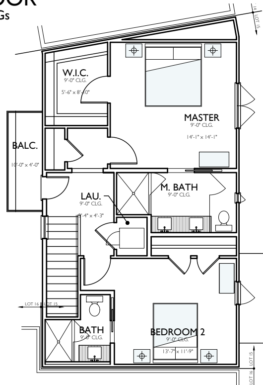
3RD FLOOR 9'-0" CLGs
