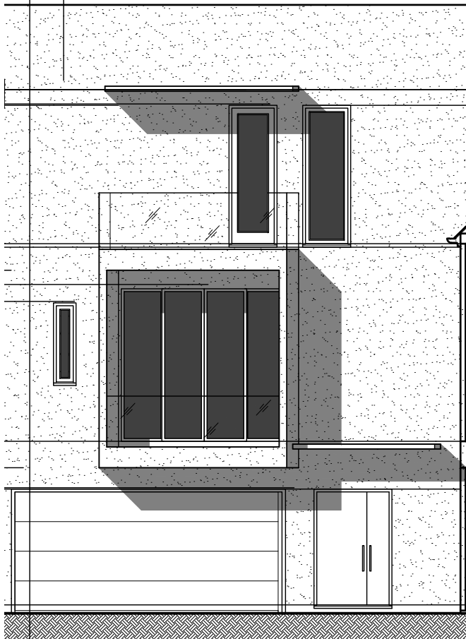
COURTYARD ELEVATION UNIT 15
