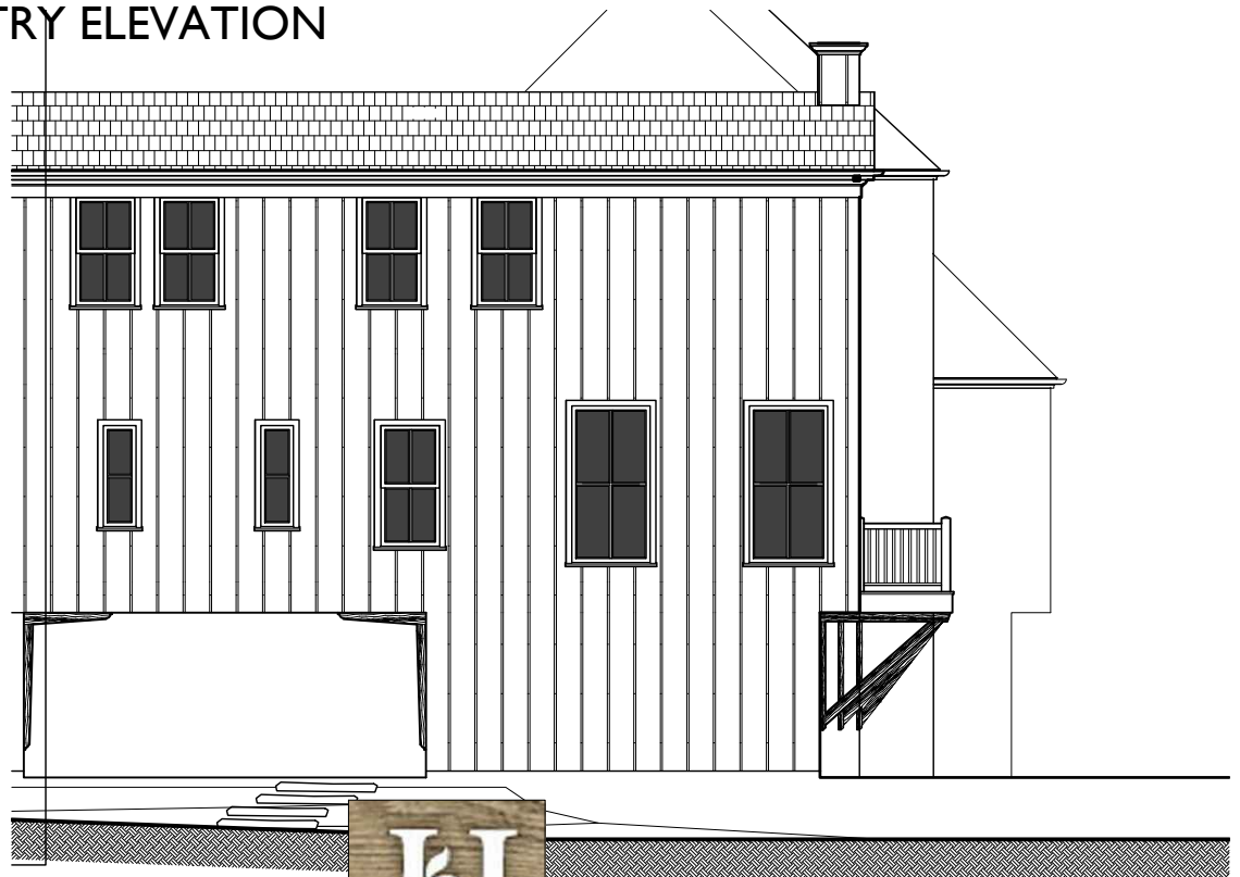
OUTER ELEVATION
