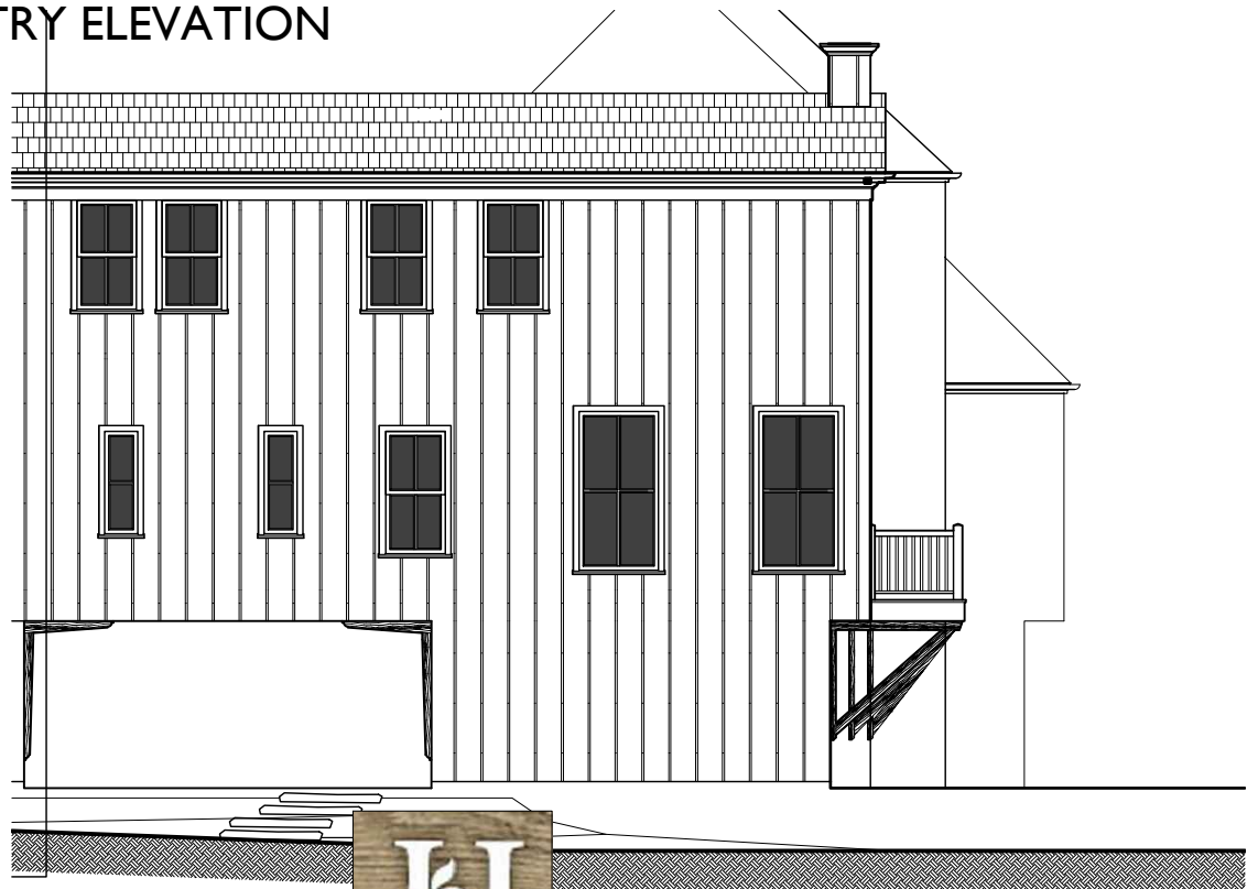
OUTER ELEVATION
