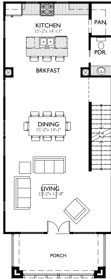
2ND FLOOR 10'-0" CLGs
