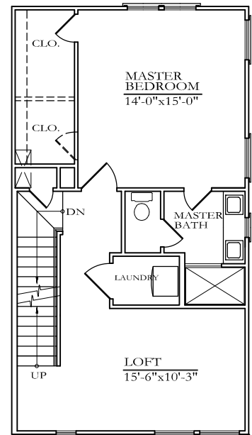
SECOND FLOOR PLAN 9'-0" CEILING
