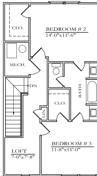
THIRD FLOOR PLAN 8'-0" CEILING
