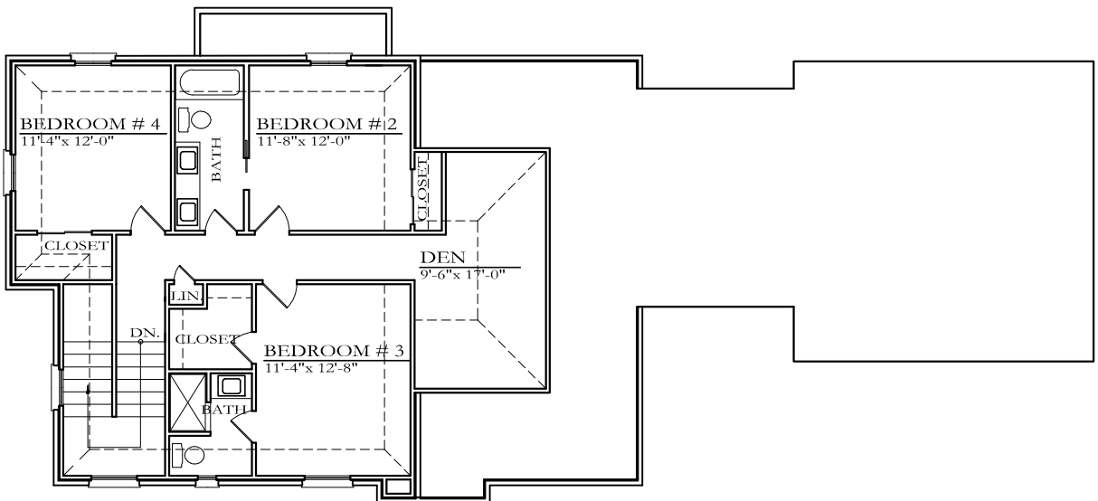
UPPER LEVEL FLOOR PLAN VAULTED 10'-0" CEILING
