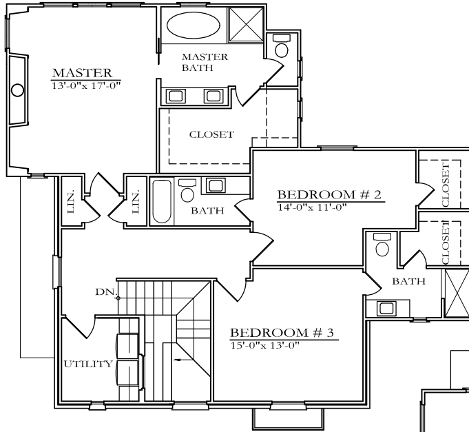
UPPER LEVEL FLOOR PLAN 9'-0" CEILING
