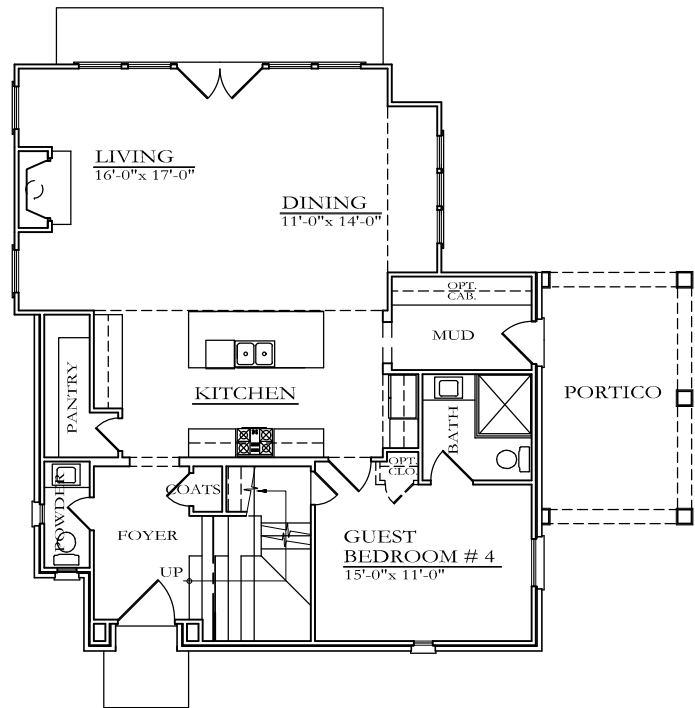
MAIN LEVEL FLOOR PLAN 10'-0" CEILING
