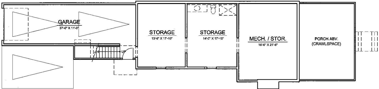
TERRACE FLOOR PLAN 8'-0" CEILING
