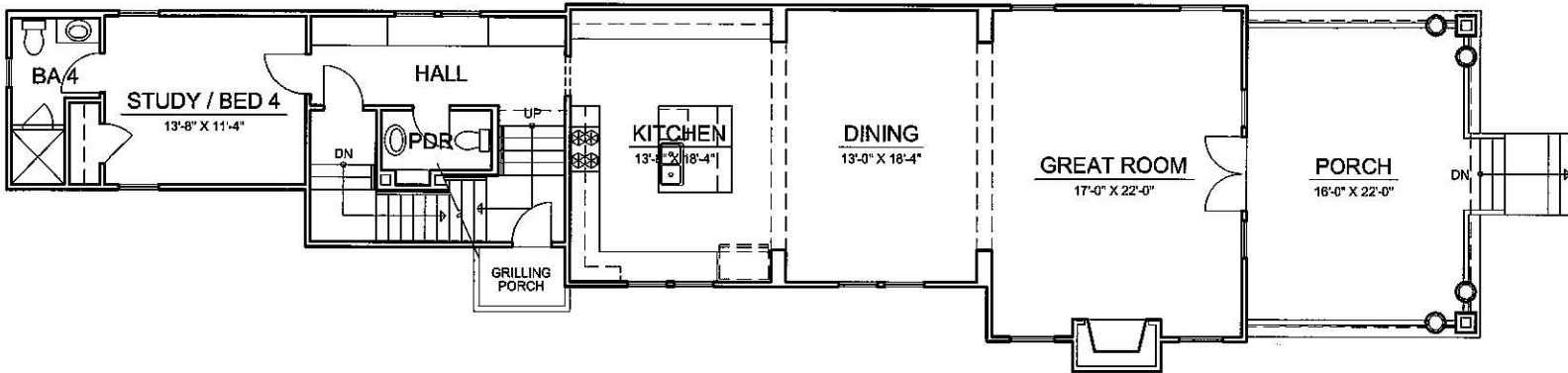
MAIN FLOOR PLAN 10'-0" CEILING
