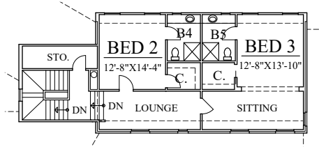
UPPER FLOOR PLAN 9'-0" CEILING
