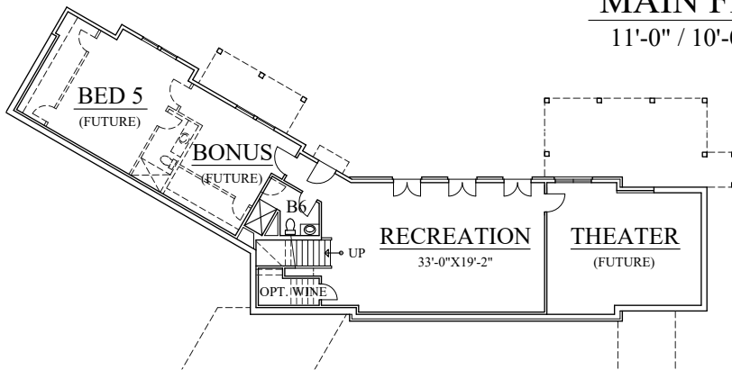
TERRACE FLOOR PLAN 9'-0" CEILING
